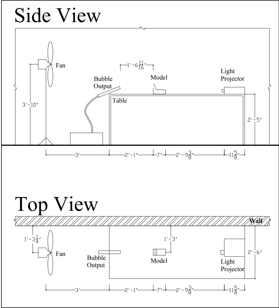
Fig. 1: Experiment General Setup.
